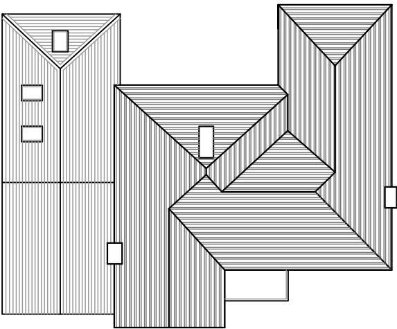
ROOF PLAN @ 1:100
