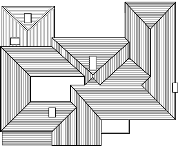
ROOF PLAN @ 1:100
