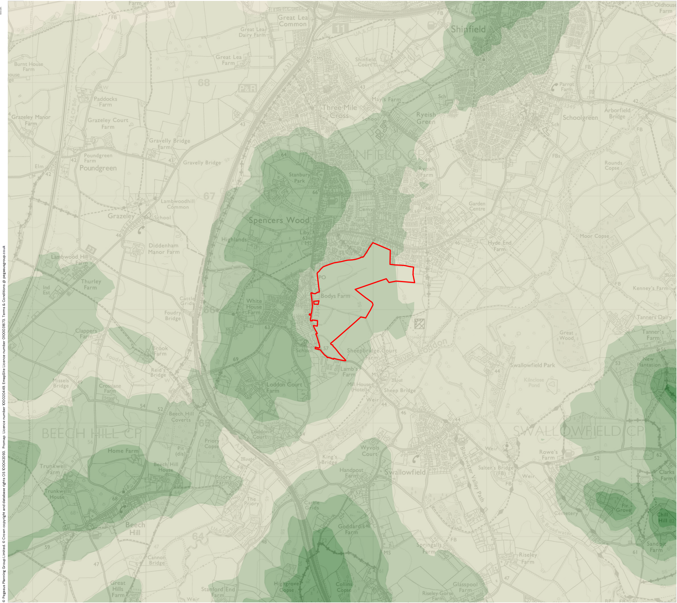
Figure 5.3: Topography
