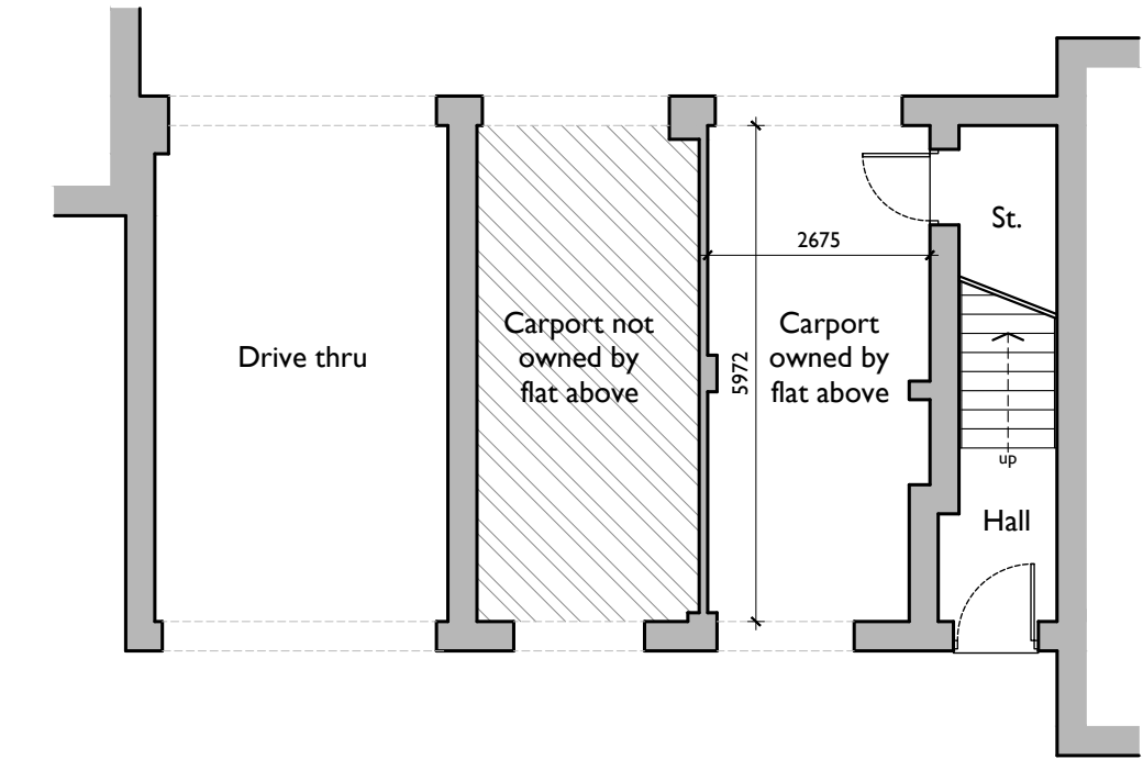
Ground Floor Layout: 1:100 at A3
