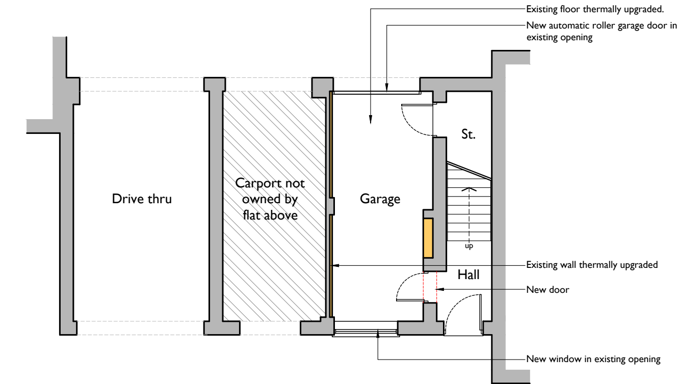
Ground Floor Layout: 1:100 at A3 0m 1m 2m 5m
