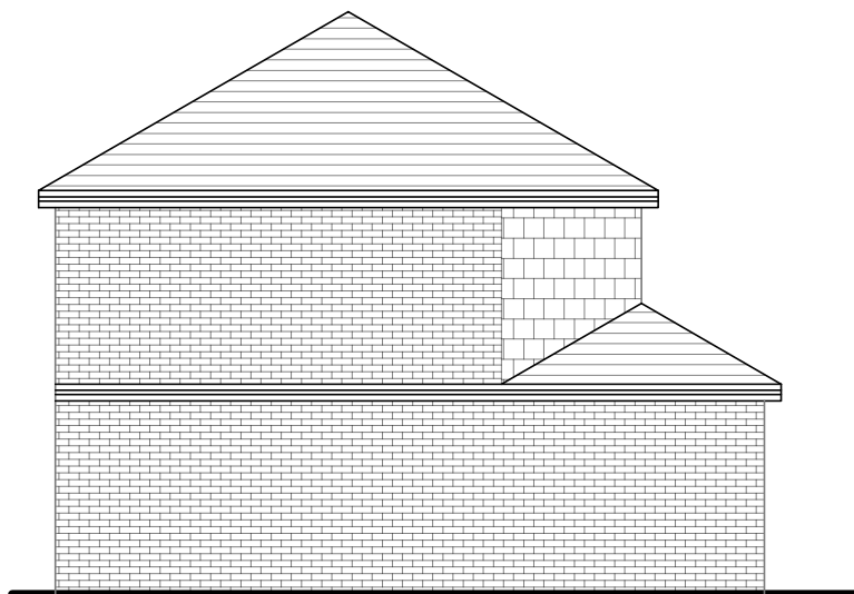
EXISTING SIDE ELEVATION (FROM NO.1) SCALE 1/100
