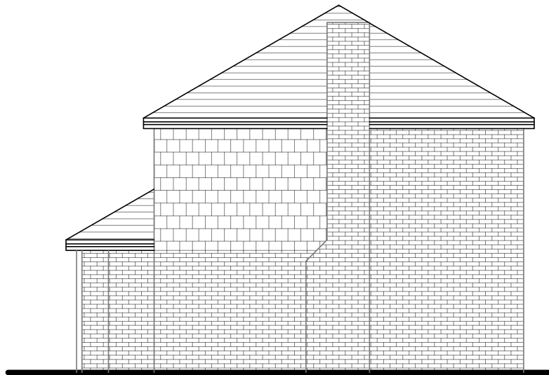
EXISTING SIDE ELEVATION (FROM NO.3) SCALE 1/100
