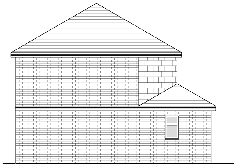
PROPOSED SIDE ELEVATION (FROM NO.1) SCALE 1/100
