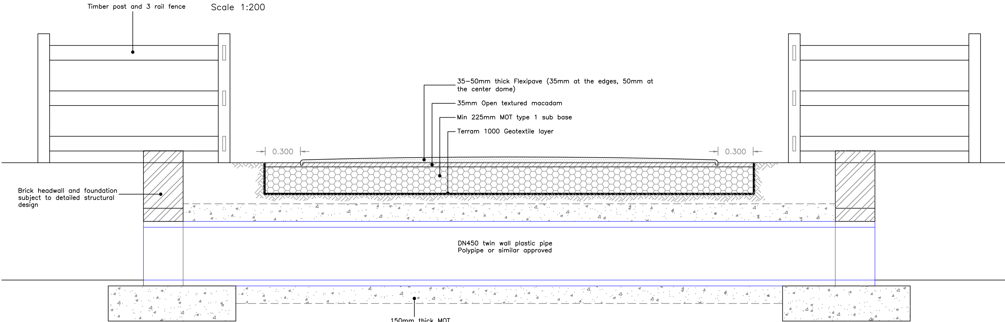
TYPICAL SECTION THROUGH CULVERT AND CROSSING Scale 1:20
