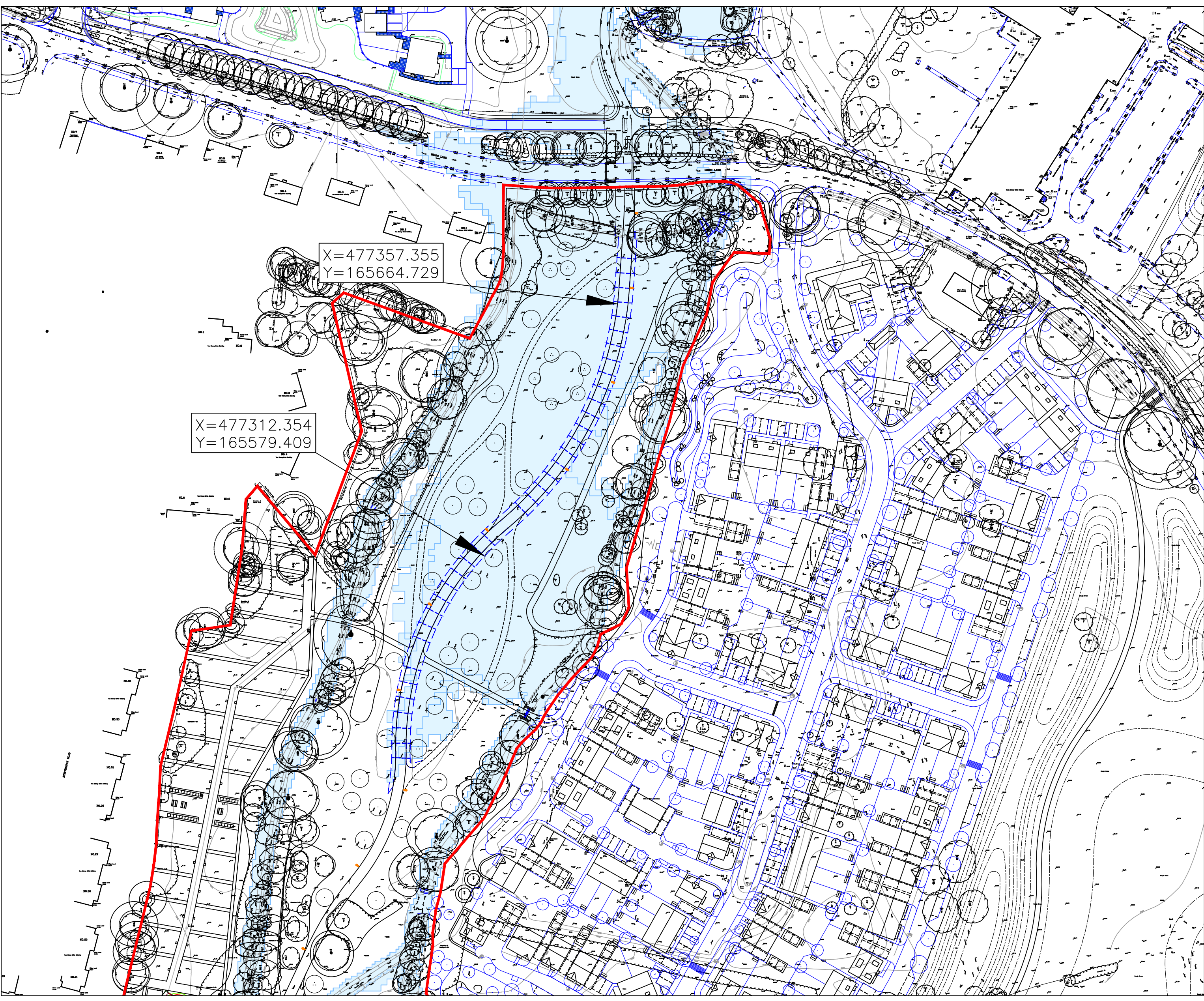
LOCATION OF RAISED FOOTPATH/CYCLEWAY WITHIN FLOOD ZONE Scale 1:1000
