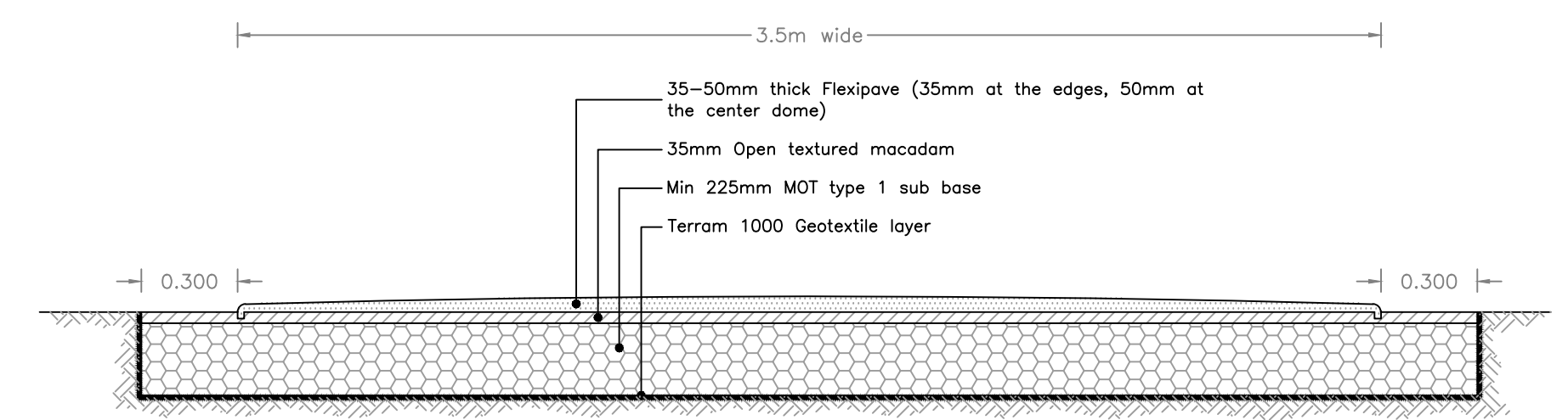
TYPICAL SECTION THROUGH 3.5m WIDE AT GRADE FOOTPATH/CYCLEWAY Scale 1:20
