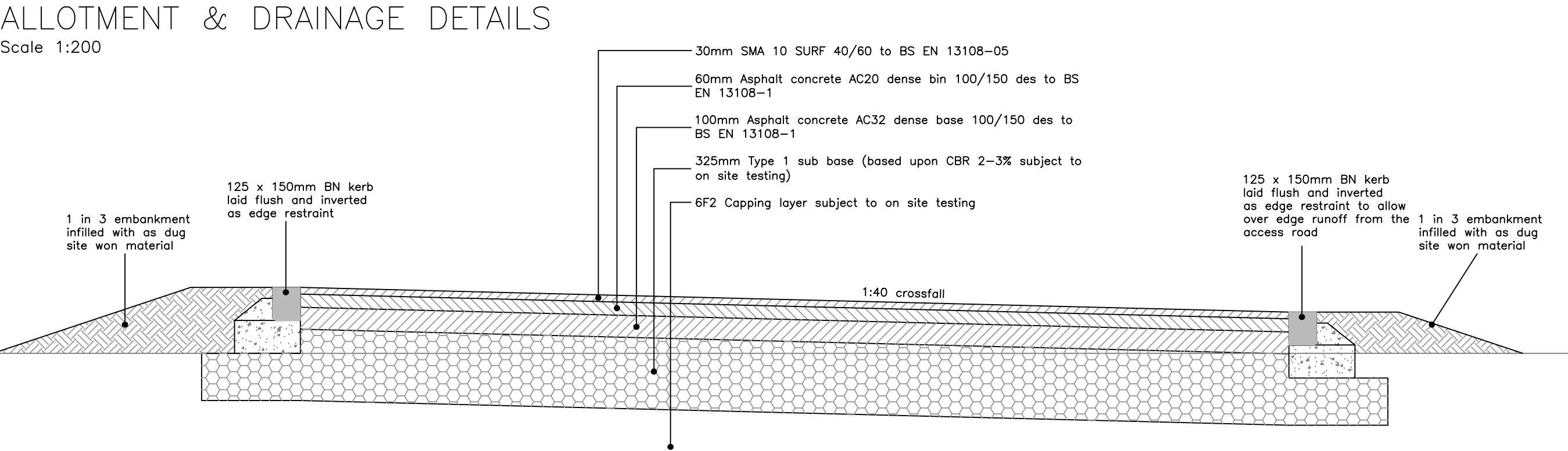
TYPICAL SECTION THROUGH 4.1m min ALLOTMENT ACCESS ROAD Scale 1:20
