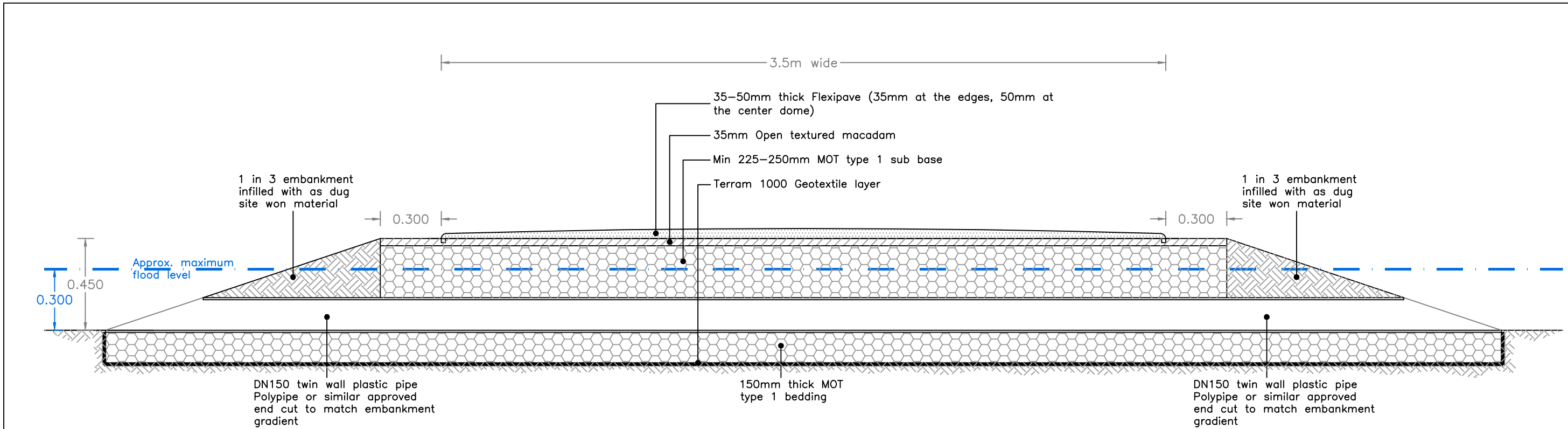
TYPICAL SECTION THROUGH 3.5m WIDE FOOTPATH/CYCLEWAY RAISED MIN 450mm ABOVE 1/100yr + cc FLOOD LEVEL Scale 1:20
