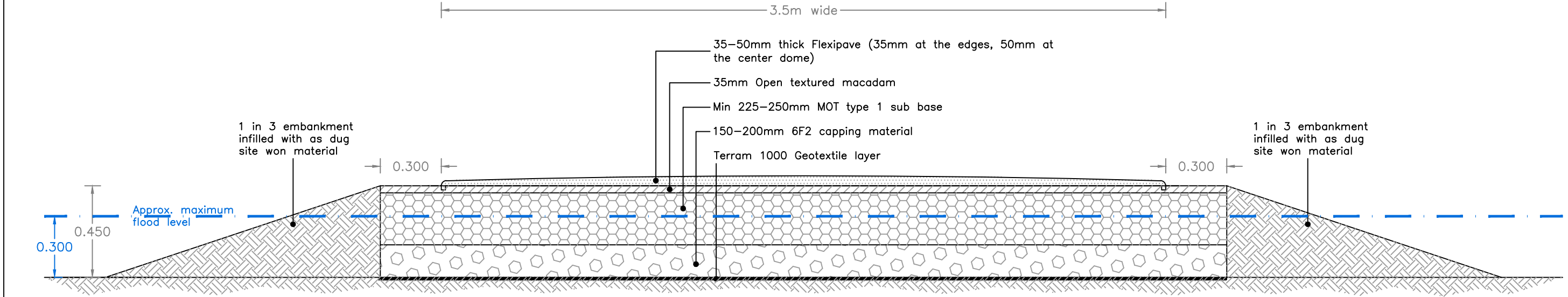
TYPICAL SECTION THROUGH 3.5m WIDE FOOTPATH/CYCLEWAY RAISED MIN 450mm ABOVE 1/100yr + cc FLOOD LEVEL Scale 1:20
